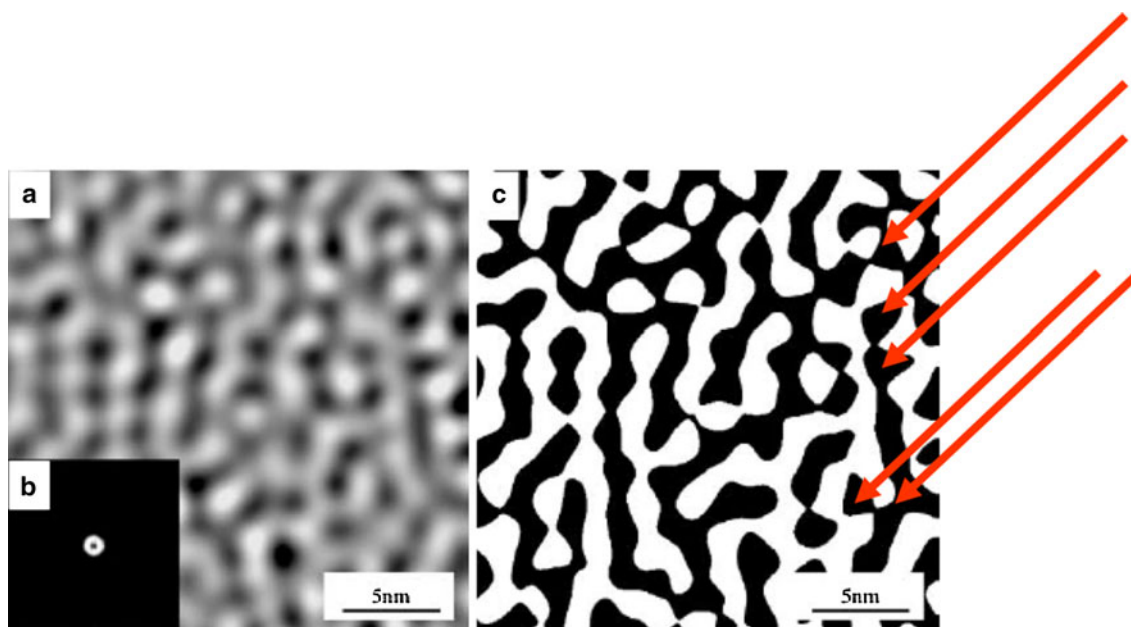
Fig. 1 High resolution TEM image of an activated carbon revealing a disordered micropore structure where many regions can be identified where an adsorbate molecule would feel a simultaneous interaction
