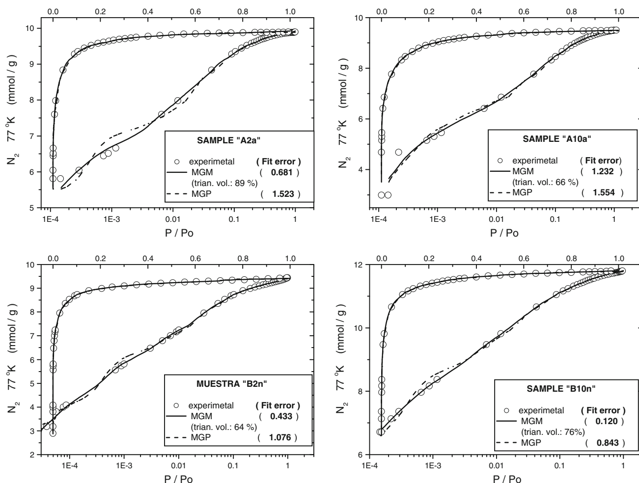
Fig. 5 N_2 77 K adsorption isotherms of samples shown in Fig. 2 and the model fit (Soares Maia et al. 2010). It is reported the percentage of “triangular” pore volume in the MGM fit (100 % level is completed by “slit” volume)
