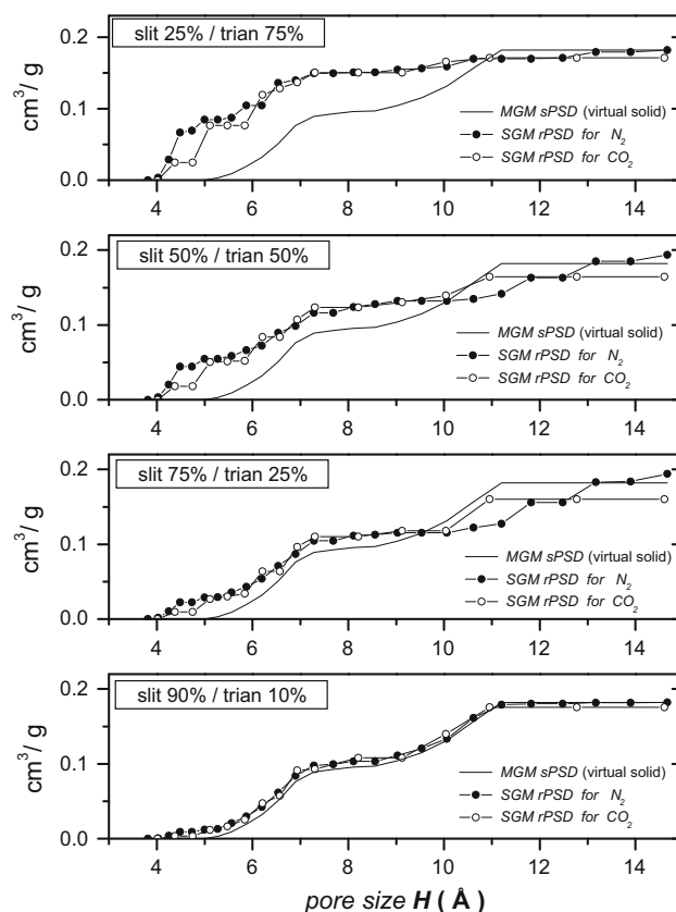
Fig. 4 Comparison between cumulative rPSDs ( N_2 77 K and CO_2 273 K) and cumulative sPSDs for virtual samples with different proportions of slit and triangular pores. The distributions tend to overlap as the proportion of slit ( triangular ) pores volume increase(decreases)
